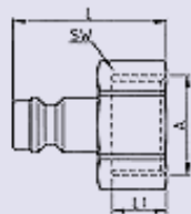
Female Thread
